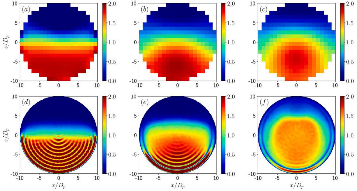
Fig. 8. Normalized mean concentration distribution, \bar{\phi}(x, z)/\phi_b , in the cross-flow plane of the pipe. (a)–(c) Experimental cases E1–E3. (d)–(f) Corresponding DNS cases D1–D3.
