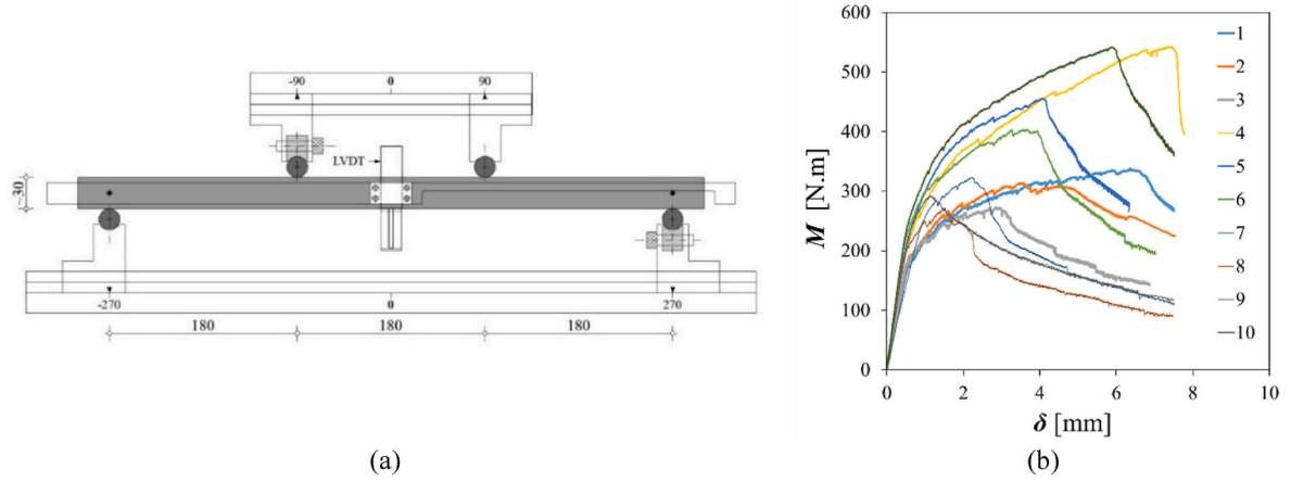
Fig. 25. Four-point bending test: (a) scheme of the test setup; (b) results for specimens 1 to 10.
