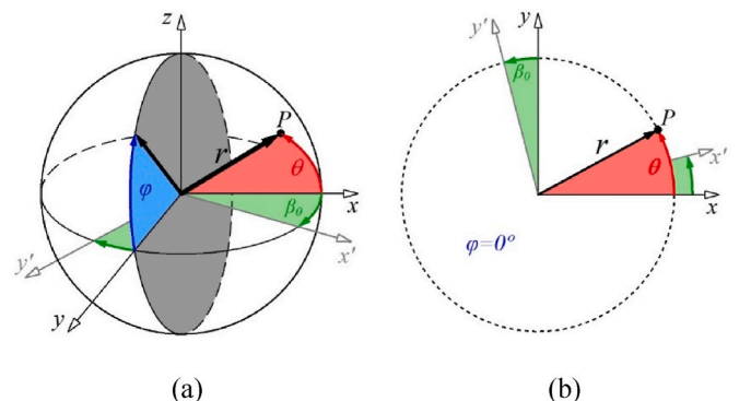
Fig. 3. Representation of fibre orientation in (a) 3D and (b) 2D.
