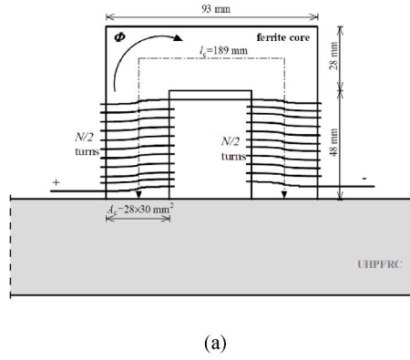
Fig. 6. NDT method (a) schematic representation of the magnetic circuit constituted by probe and UHPFRC layer [65]; and (b) measurements on a UHPFRC thin element.
