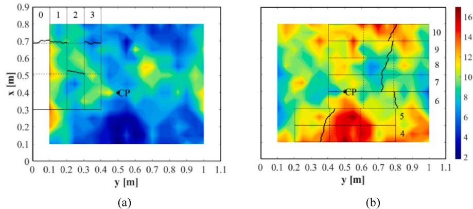
Fig. 24. NDT tensile strength [MPa] contour maps and FPBT cracks of LP1 (a) f_{Uti,x} and (b) f_{Uti,y} .
