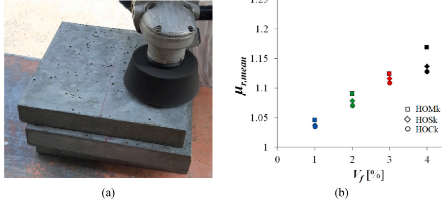
Fig. 20. Surface effect on \mu_{r,mean} : (a) mechanical smoothing of the casting surface; (b) regression lines for the different surface types.
