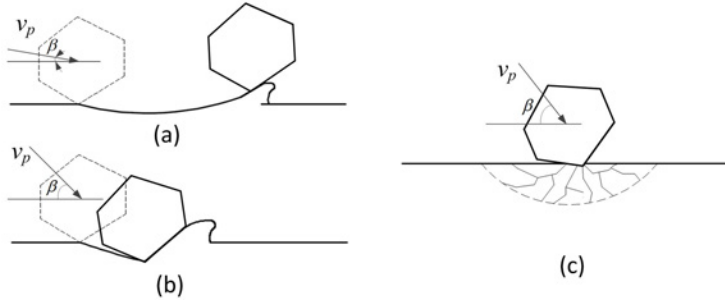
Figure 2.8: Schematic illustration of erosive wear (a) low angle impact (b) high angle impact (c) brittle fracture caused by particle impact [33]
