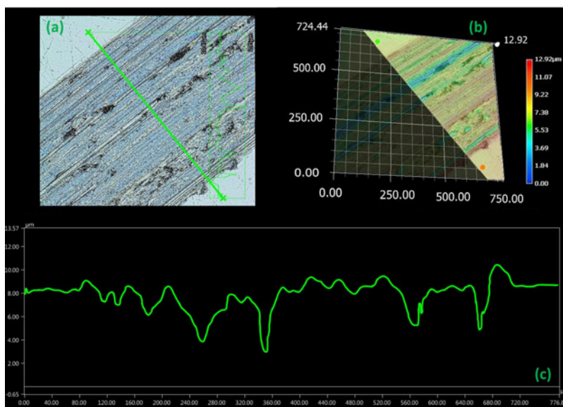
Figure 4.13: Wear morphology of a mild steel disk surface (a) an area of wear path; (b) 3D visualization; (c) profile of the measured cross-sectional area
