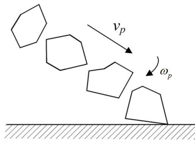
Figure 2.7: Schematic illustration of erosive wear in bulk solids handling
