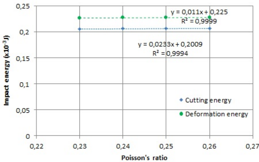
Figure 5.26: Impact wear energy as a function of particle Poisson's ratio
