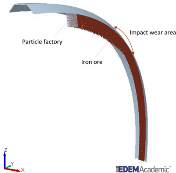
Figure 7.1: Simulation model for predicting erosive wear
