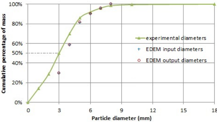
Figure 6.1: Particle size distribution for the wear modeling
