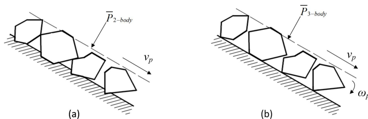
Figure 2.5: Schematic illustration of abrasive wear (a) two-body abrasion or sliding wear (b) three-body abrasion
