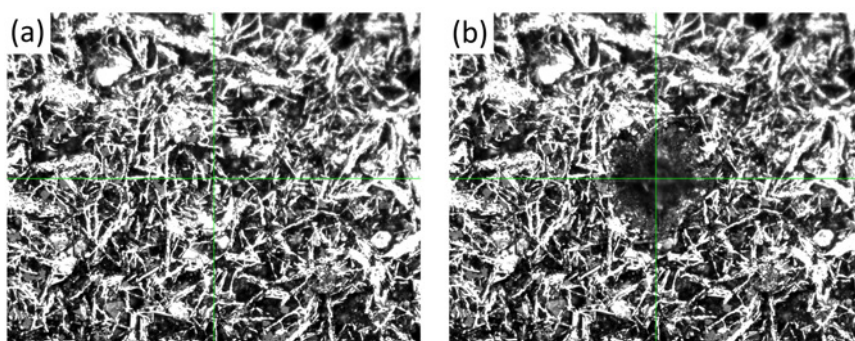
Figure 4.5: Surface texture of a Sishen particle (a) before test (b) after test (400 \times )
