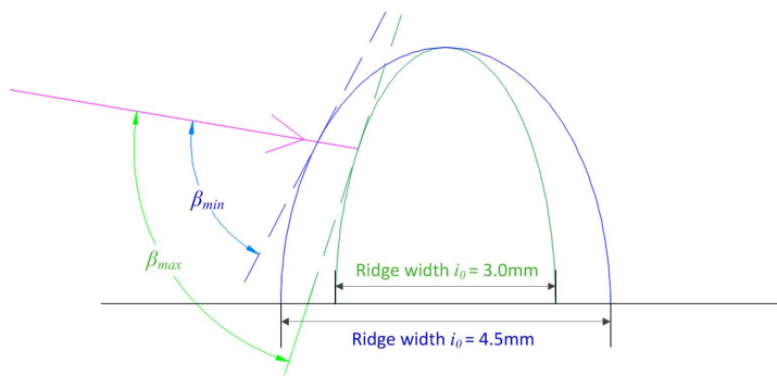
Figure 7.16: Variation of impact angle by increasing ridge width i_0
