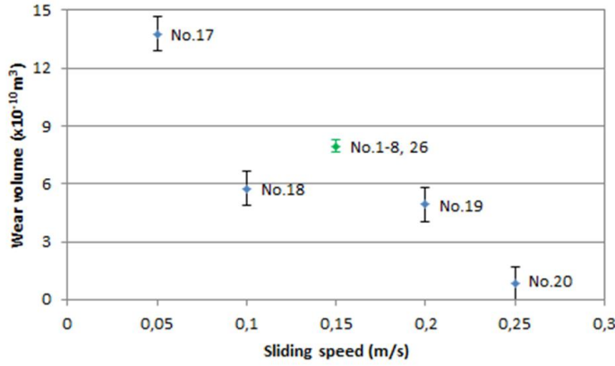
Figure 4.20: Wear volume of particle as a function of siding speed
