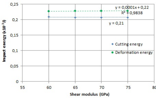
Figure 5.27: Impact wear energy as a function of particle shear modulus
