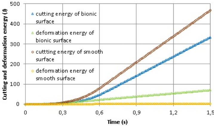
Figure 7.6: Comparison of cumulative cutting and deformation energy ( group 2 )
