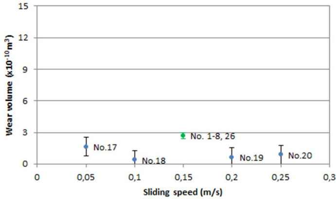
Figure 4.21: Wear volume of mild steel as a function of siding speed
