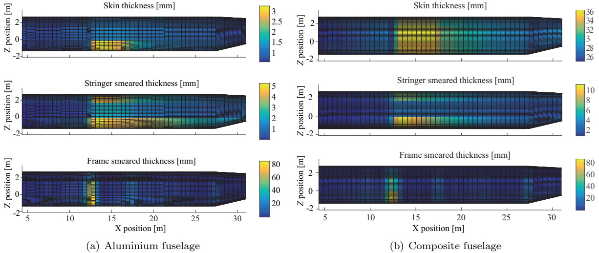
Figure 13. Airbus A320-200 thickness distribution
