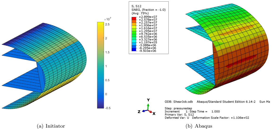
Figure 10. Shear Stress
