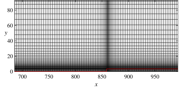
Fig. 12. Grid lines indicated in black. One in every forty \xi and one in every eight \eta lines are shown. The step surface is indicated in red.
