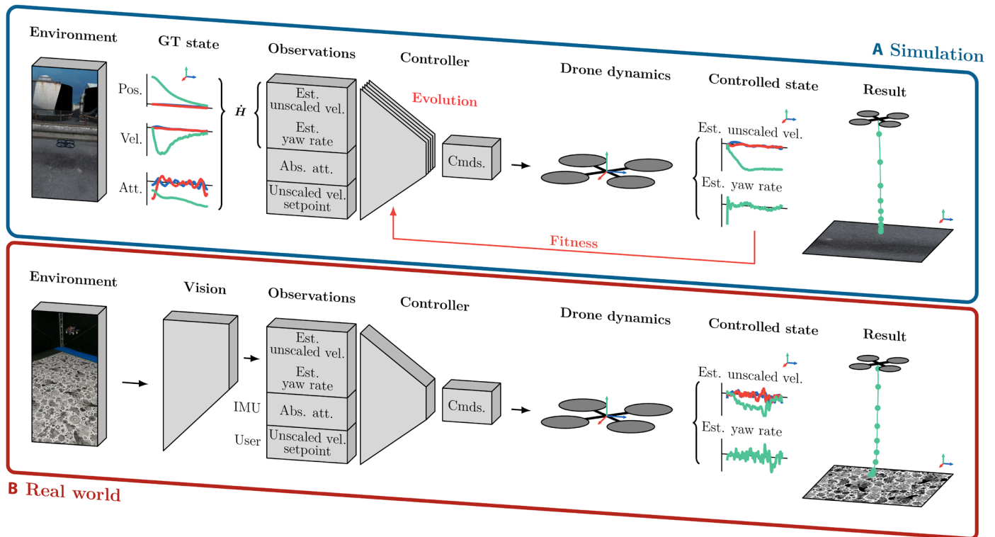
Fig. 3. Overview of the control pipeline for simulation and real-world tests. During training in simulation ( A ), we constructed visual observables (unscaled velocities and yaw rate) from ground truth using the continuous homography transform. The control decoding takes these observables together with roll and pitch and an ego-motion set point to output commands, which control the drone dynamics. We have trained the controller using evolution on the basis of a fitness signal that quantifies how well the controller can follow ego-motion set points for horizontal and vertical flight. In the real world ( B ), we receive flows of the corner ROI from the vision network and transform these to visual observables and control commands in a single matrix multiplication to send low-level control commands thrust and attitude to the autopilot.
