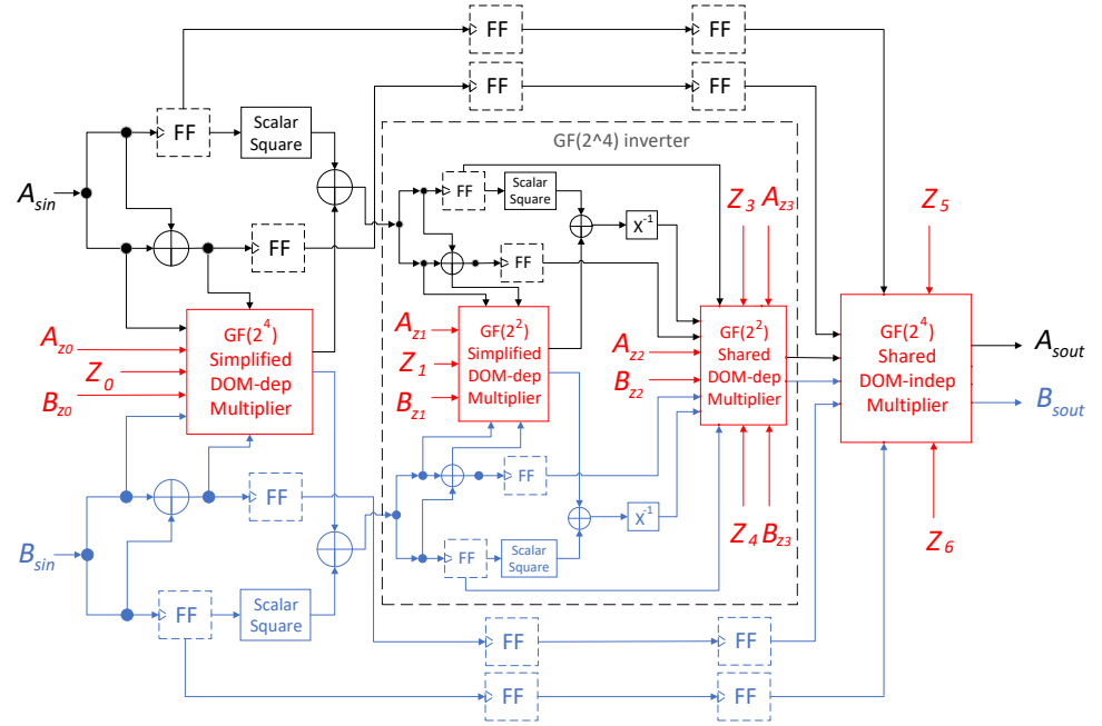
Figure 9. Structure of the first-order 5-pipeline-stage DOM SBOX shared module.
