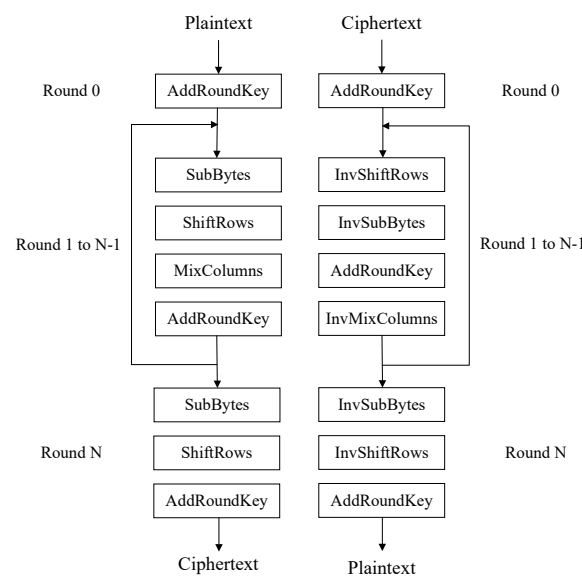
Figure 1. AES encryption and decryption flow diagram.
