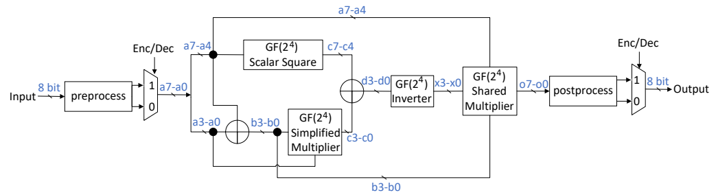
Figure 5. Proposed shared SBOX.
