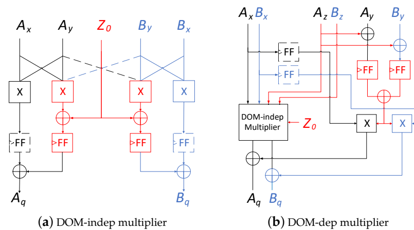
Figure 2. First-order DOM-indep and DOM-dep multipliers [15].
