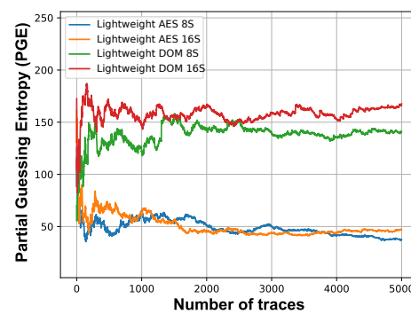
Figure 14. Template-based security analysis of unprotected and proposed designs.
