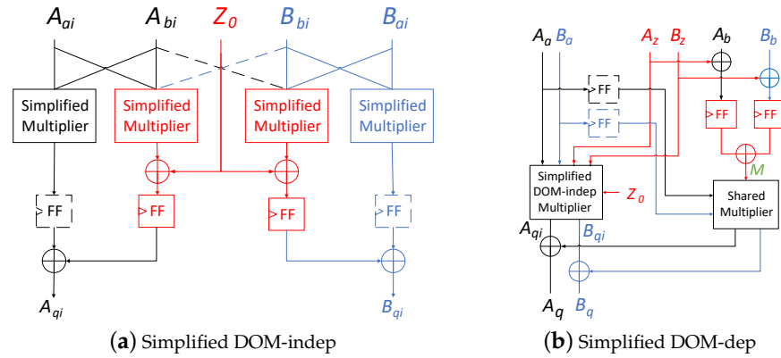
Figure 10. Proposed first-order simplified DOM-indep and DOM-dep multipliers
