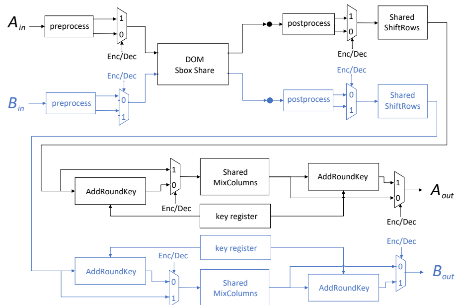
Figure 8. Proposed design for DOM encryption and decryption.
