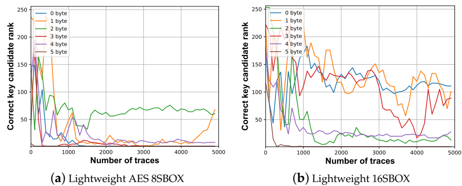
Figure 12. Rank analysis of the lightweight implementations for the FPGA.
