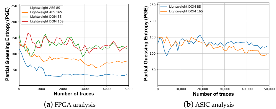
Figure 11. Security analysis of unprotected and proposed designs.
