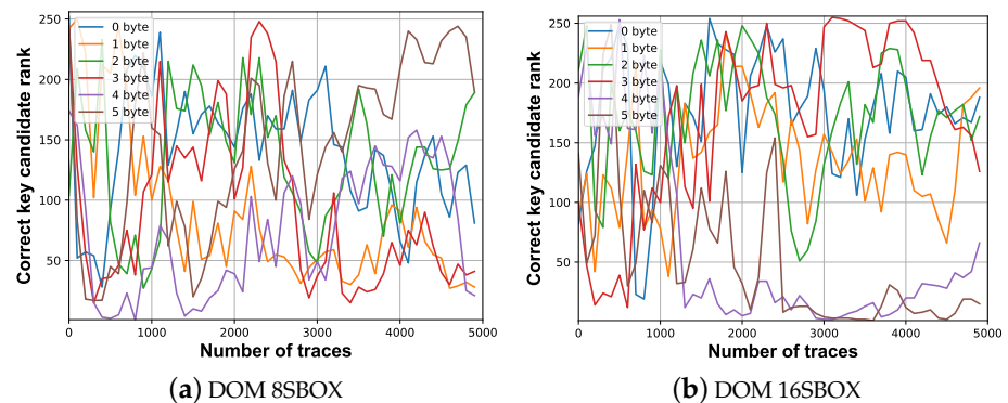
Figure 13. Rank analysis of the DOM-based lightweight implementations for the FPGA.
