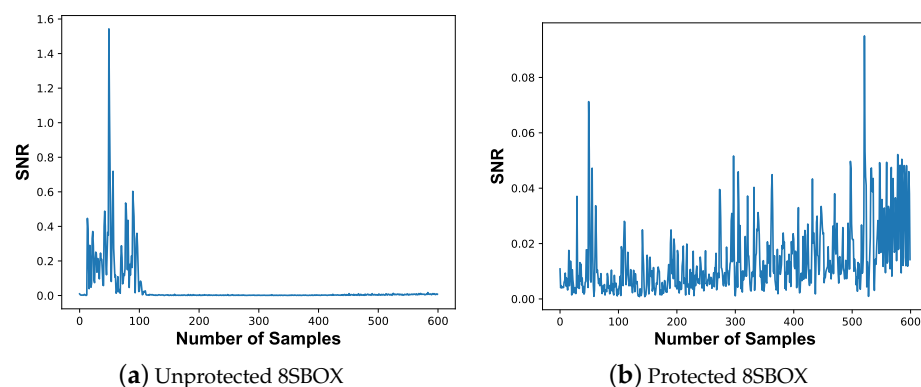
Figure 15. SNR analysis.
