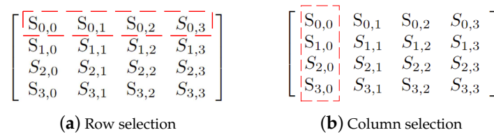
Figure 3. Input selection example in 32-bit design.
