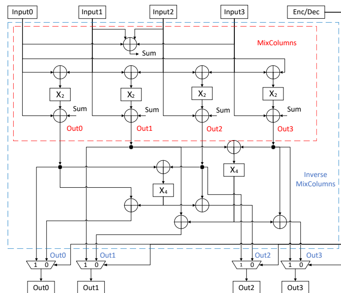
Figure 7. GF(2^4) shared MixColumns.
