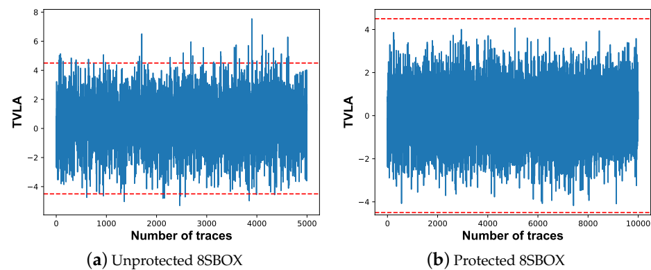
Figure 16. TVLA analysis.
