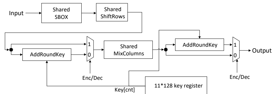
Figure 4. Proposed round function AES encryption and decryption.
