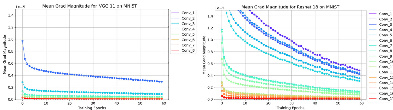
Fig. 1 The graphs represent the average absolute partial derivative (AAPD) value of each convolutional layer in the VGG-11 (left) and ResNet-18 (right) on the MNIST dataset (AAPD on the y-axis, epochs on the x-axis). Each curve represents a different layer (purple for
