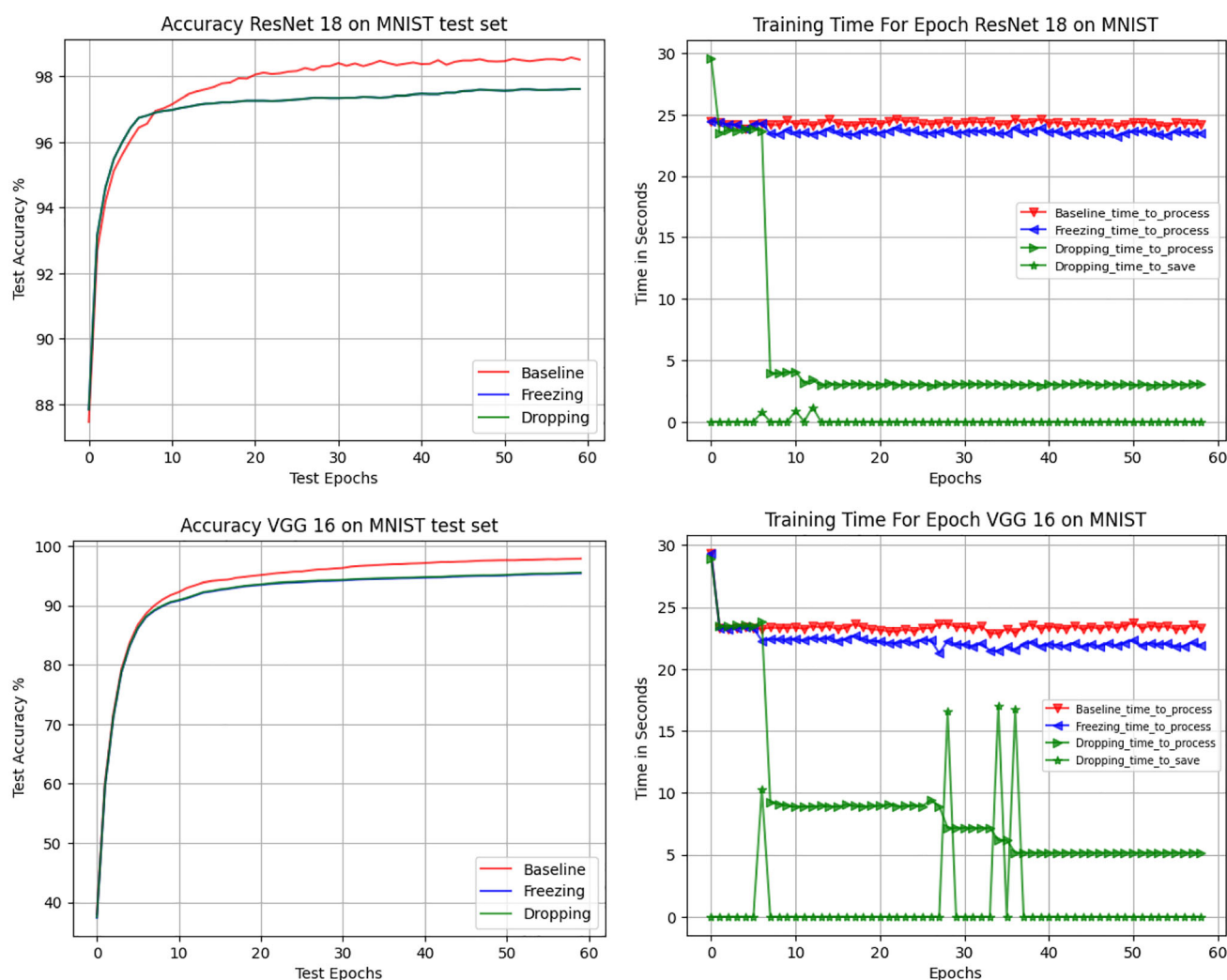
Fig. 5 The plots on the left show the test accuracy values of a ResNet-18 (top) and VGG-16 (bottom) trained on the MNIST dataset with different strategies: SGD (red curves), layer freezing (blue curves), and layer dropping (green curves). The experiments were repeated 10 times with different starting weights and data randomization. Freezing and dropping layers achieve nearly equivalent test accuracy values,
