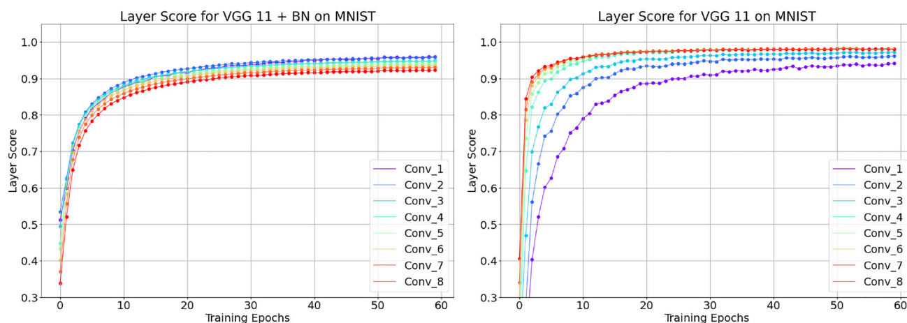
Fig. 3 The plots show the scores P_l^{(k)} on the MNIST dataset for a VGG-11 trained with (on the left) and without batch normalization (on the right). Batch normalization reverses the order of the score
