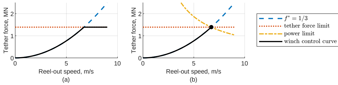
Figure 3: Winch control curves for the two control strategies. The optimal torque control strategy (a) follows the optimal reel-out factor until the tether force limit is reached and then aims to keep the tether force constant. The kite tether force control strategy (b) follows the optimal reel-out factor until the tether force and power limit are reached and then aims to stay at those limits by using kite tether force control.
