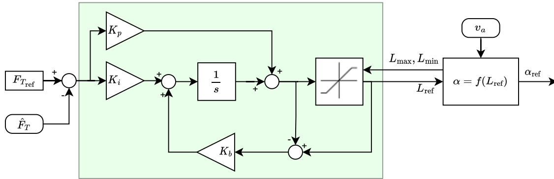
Figure 4: Block diagram of the kite tether force controller. From the tether force error a PI controller with anti-windup outputs a reference lift force that is then converted to a reference angle of attack by inverting the linear lift curve. The safe bounds on angle of attack are used to saturate the PI controller.
