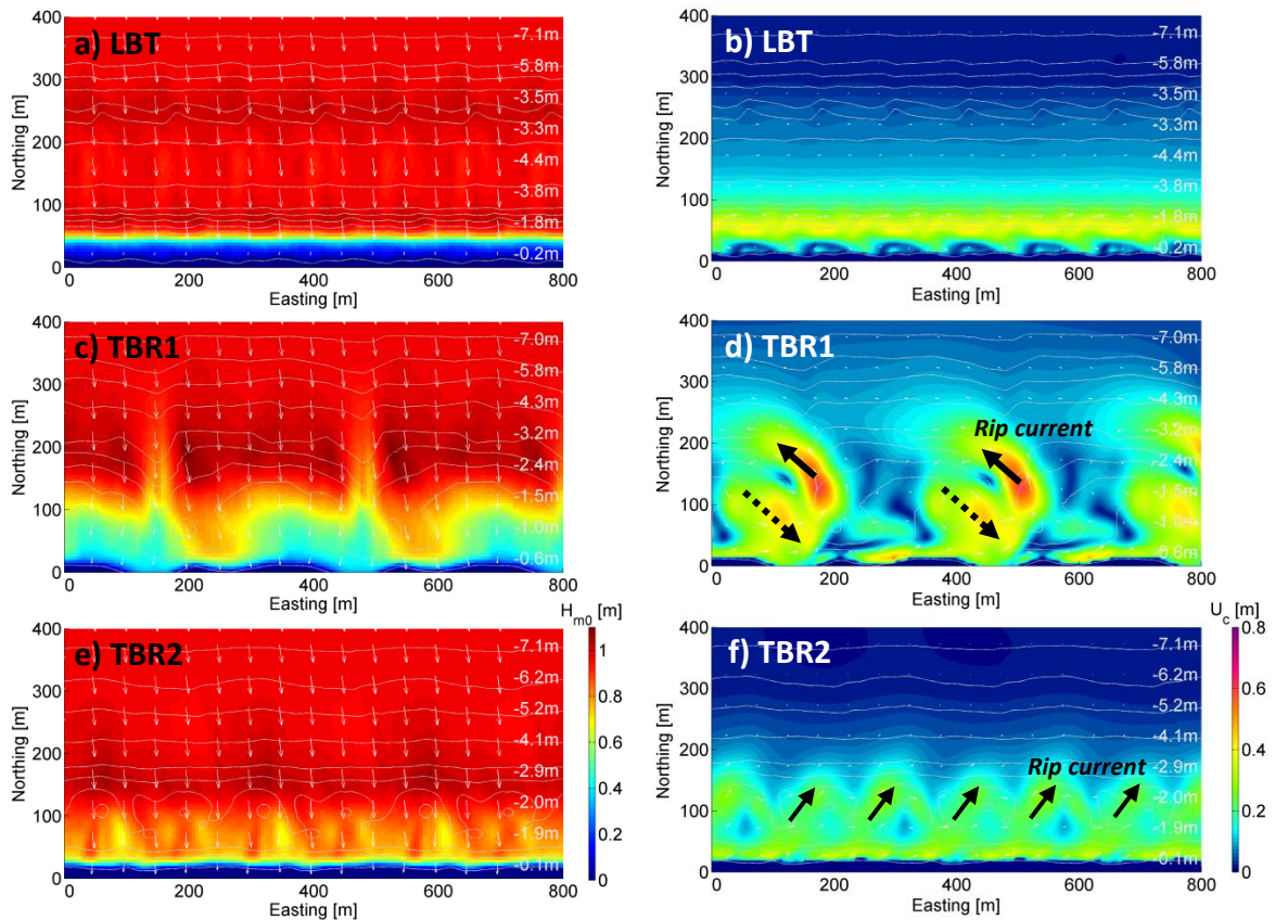
Figure 4 : Hydrodynamic conditions for the LBT, TBR1 and TBR2 beach states for a moderate wave condition ( H_s=1 m, T_p=6 s and \theta=350^\circ N). Depth contours of the bathymetry are shown in gray. Left panels: Significant wave height; Right panels: Velocity magnitude.
