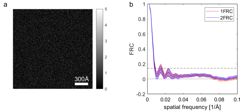
Fig. 7. Single and double image FRC for TEM. (a) Example image indicating the very low signal values of TEM data. (b) Corresponding single ("1FRC") and double ("2FRC") image FRC curves. Both the mean FRC curves and the spread quantified by the standard deviation over the M = 25 curves are plotted. The FRC resolution values were a comparable 42.4 \pm 2.1 Å (1FRC) and 43.6 \pm 2.3 Å (2FRC).
