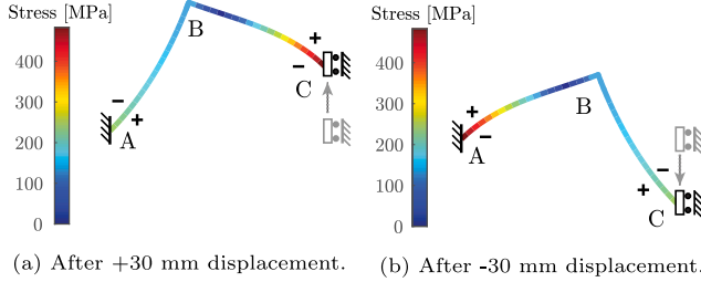
Fig. 10. FEM simulations showing high peak stresses (482.6 MPa) in the traditional FLS at large displacements.
