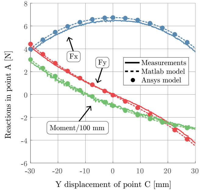
Fig. 14. Experimental results of the redesigned FLS, compared to the two FEM models, showing a maximum NMAE of 5.5%.
