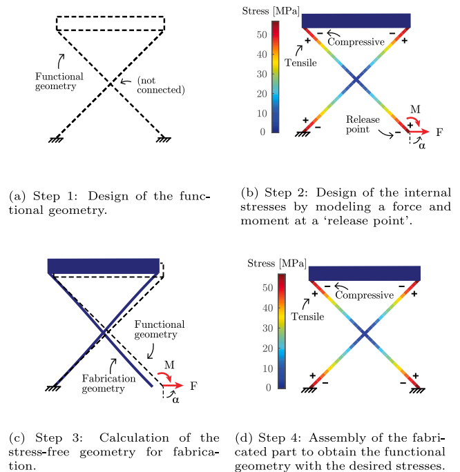
Fig. 3. The four steps of the STAGE method, explained with the crossed-flexure pivot. The geometry in the last step is the same as in the first step and exhibits the desired stresses.
