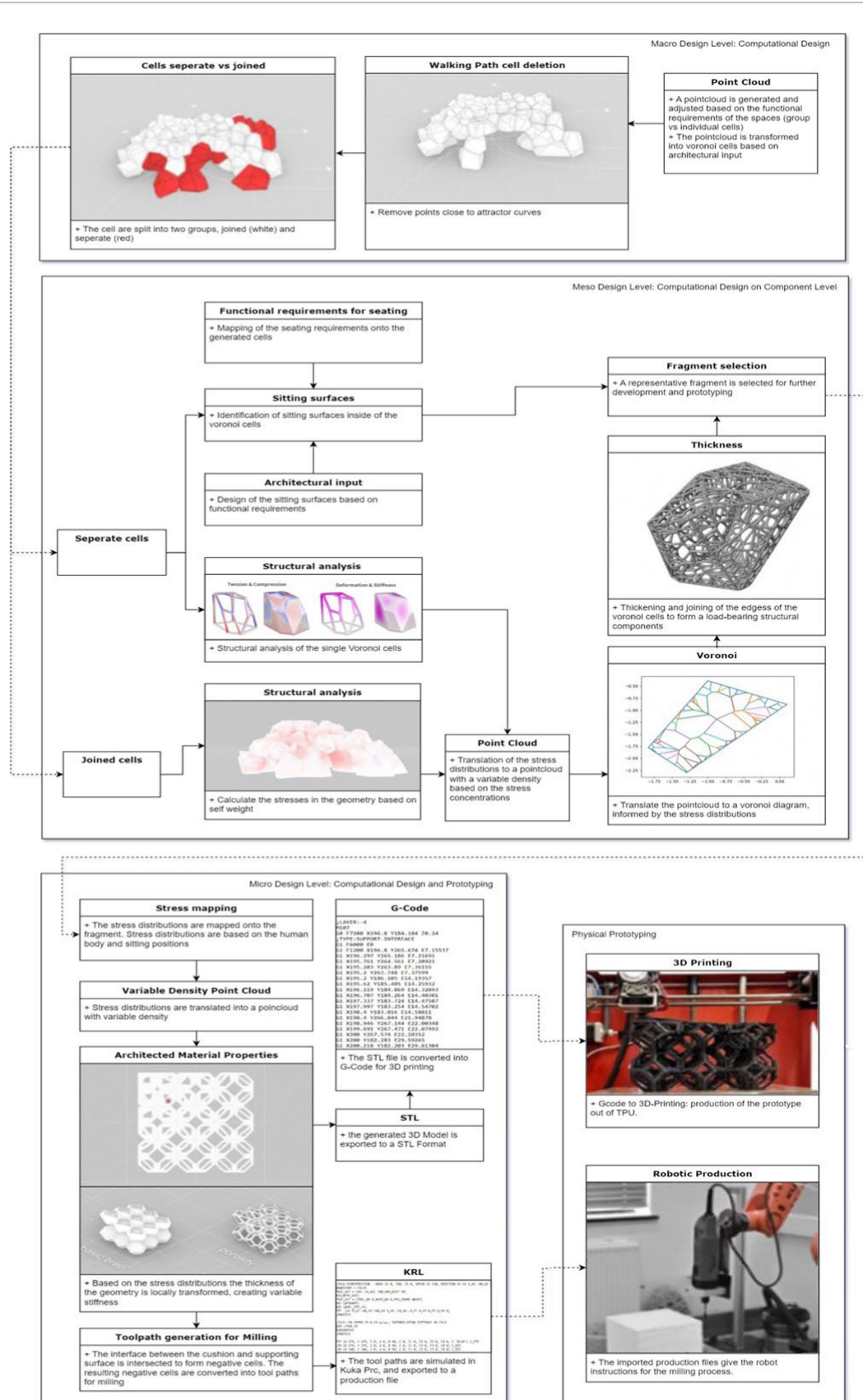
FIGURE 8 Diagram showing D2RP process reaching prototyping level.
