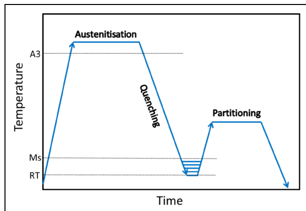
Figure 1. Applied Q&P heat treatments on LMn and HMn alloys.
