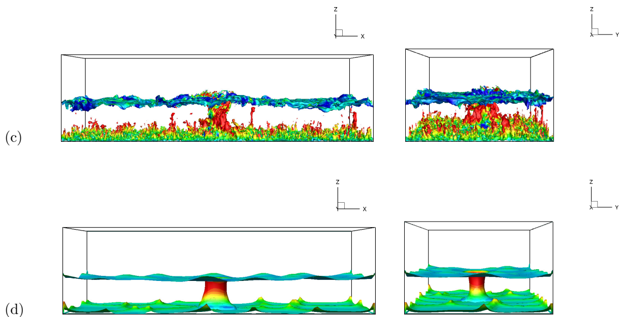
Figure 2. Iso-surface of the instantaneous non-dimensional temperature ( \theta^* ) at characteristic non-dimensional time of t^* = 200 , with two heating scenarios: Case1- uniform and Case7- nonuniform heating: (a) and (c) - LES results; (b) and (d) - TRANS (AFM) results; Left- a view in (x-z) plane; Right- a view in (y-z) plane;
