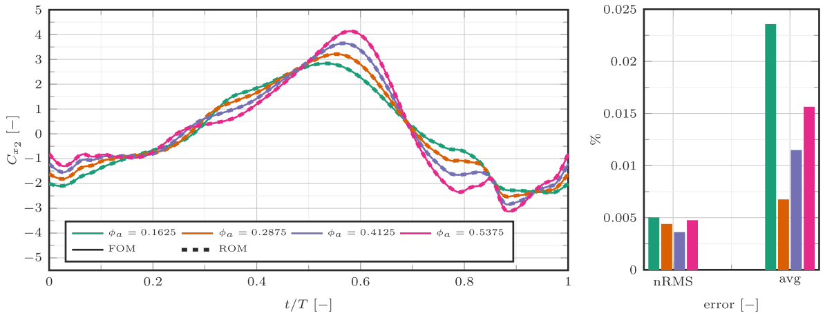
Fig. 18. Motion profile study: Horizontal force coefficient C_{x2} and corresponding normalized RMS error and absolute error of the average force for reduced-order w.r.t. full-order model.
