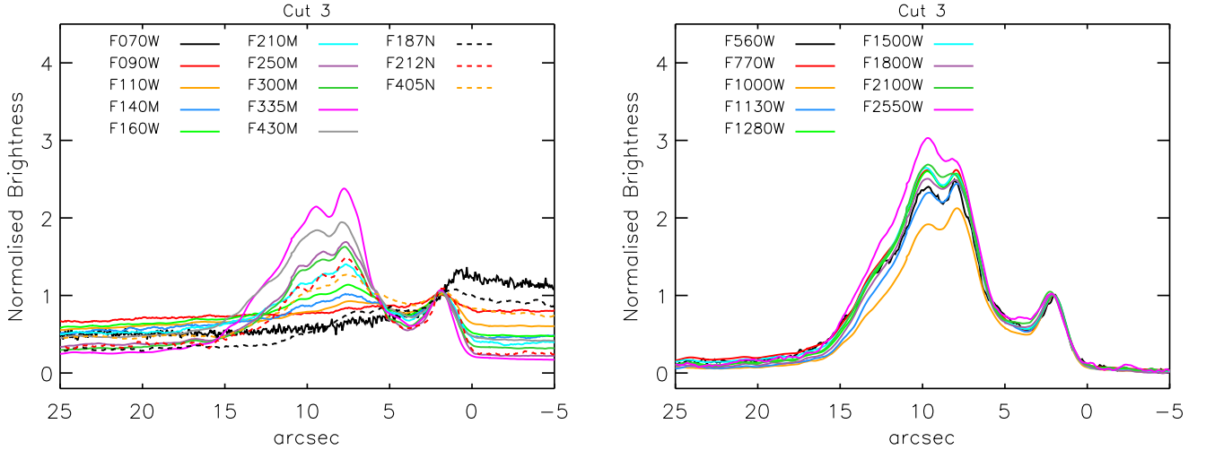
Fig. 7. Profiles of the relative brightness (normalized at a distance of 2'' from the edge) for NIRC and MIR filters for cut 3 with no background correction.
