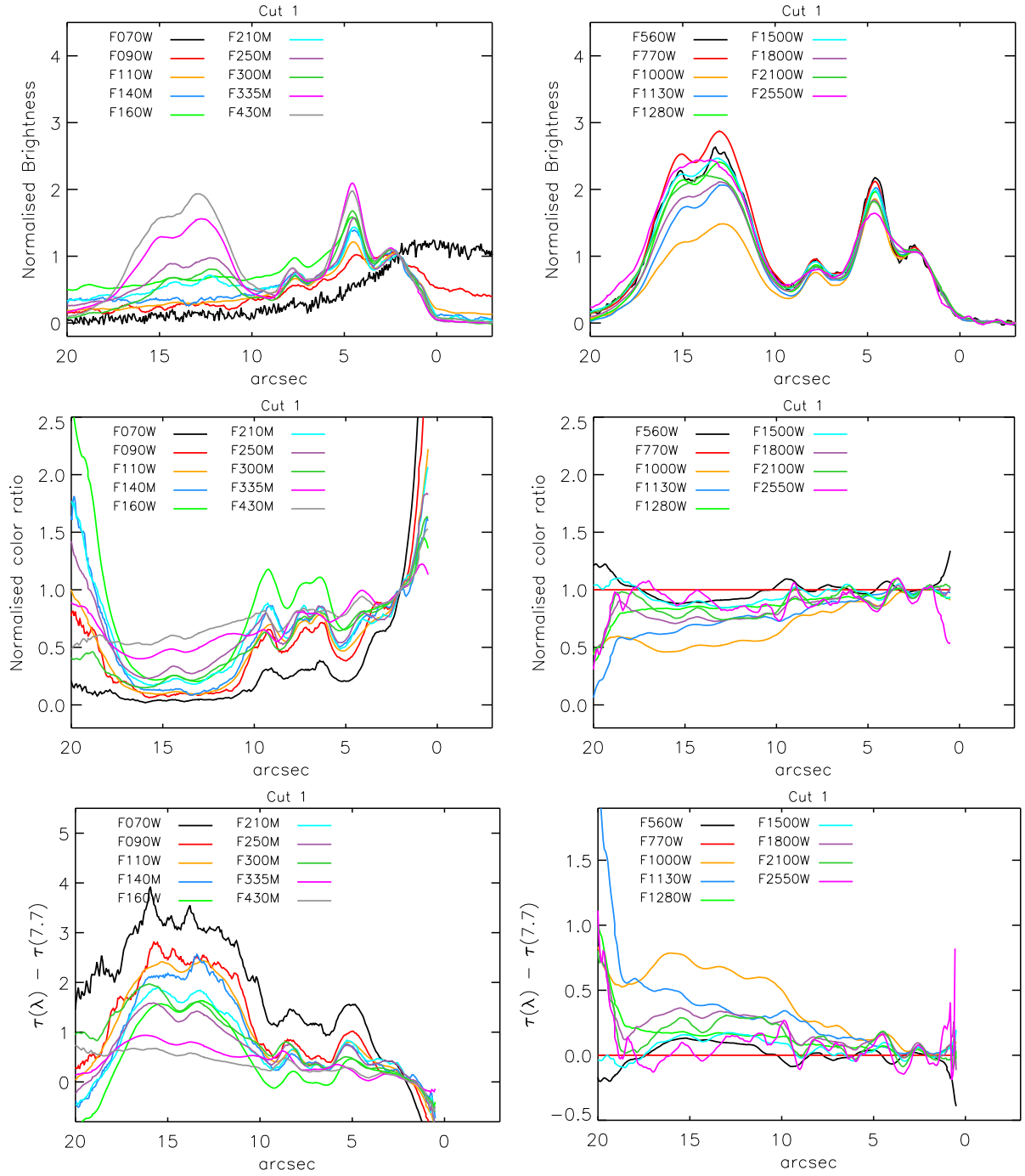
Fig. A.1: Same as Fig. 12 for cut 1
