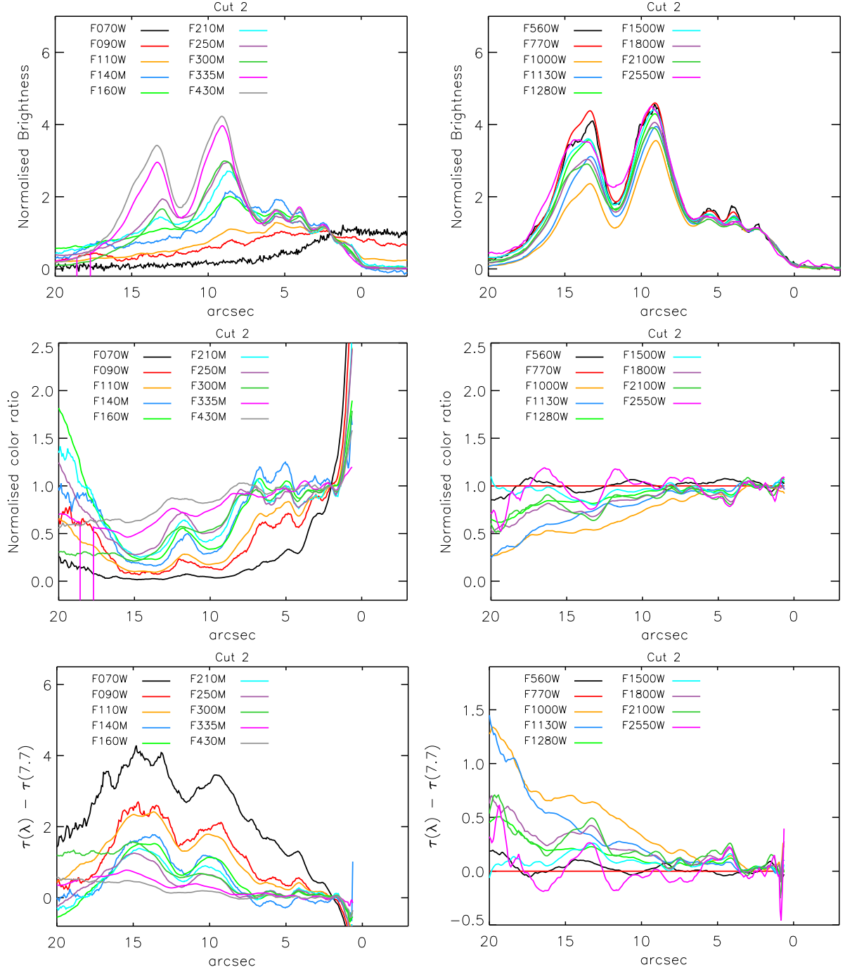
Fig. A.2: Same as Fig. 12 for cut 2
