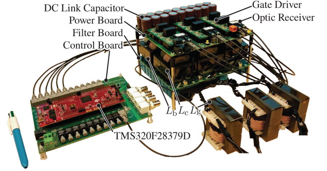
Fig. 9. Experimental setup.
