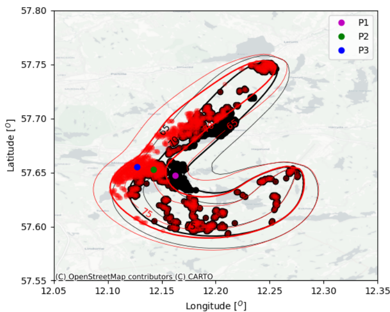
Fig. 5 SEL contour lines and population exposed to noise level higher than 70 dB(A) depicted as dots for the standard (red) and test procedure (black).
