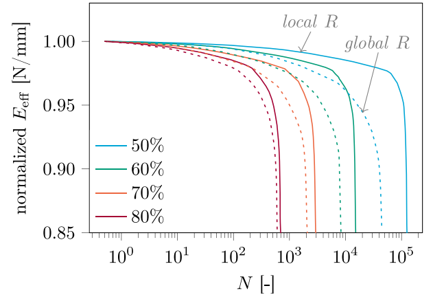
Fig. 10. Stiffness reduction with number of cycles for four different severity levels. Dashed and solid lines correspond to the response with global and local stress ratio, respectively.
