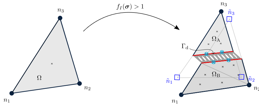
Fig. 3. XFEM crack insertion. The mixed-mode fatigue cohesive zone model is used in each cohesive integration point ( \otimes ) for describing fatigue damage.
