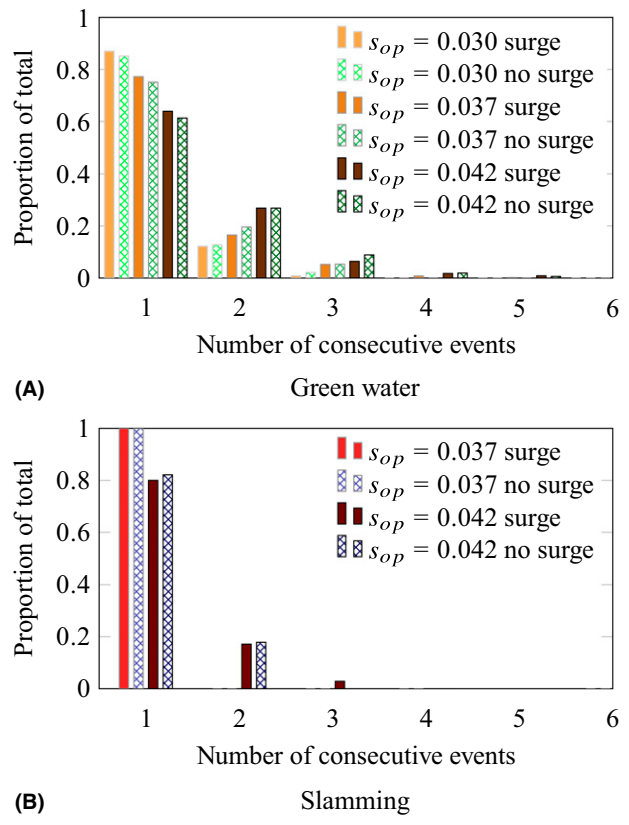
Fig. 13 Comparing the number of consecutive events for different spectral steepnesses. The average number of events per cluster is lower for a lower spectral steepness, with somewhat larger cluster sizes for test cases where the surge was restricted
