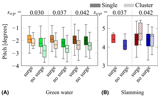
Fig. 12 The maximum pitch motion during clustered and single events are compared, showing on average larger pitch motions for clustered events than single events
