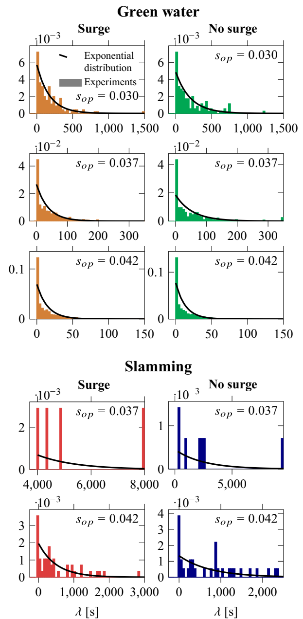
Fig. 7 Density histograms of time between events ( \lambda ) show zero inflation caused by clustering. The fitted exponential distribution does not fit the data due to the zero inflation
