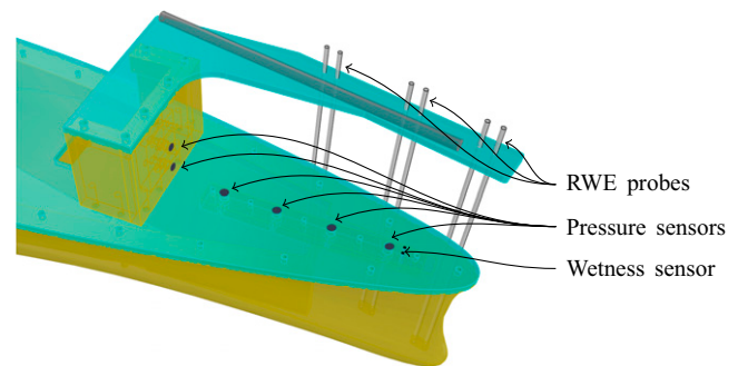
Fig. 2 Measuring equipment on the bow
