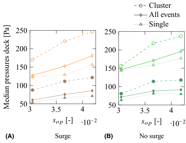
Fig. 11 On average the pressures on the deck for green water events in a cluster are larger than the pressures due to single events. The solid markers indicate the median pressures ( \bar{p}_{max} ) and the open markers the maximum ( p_{max} )
