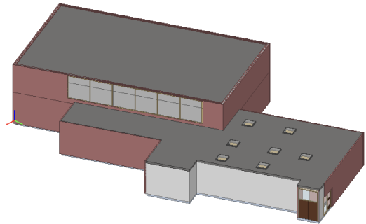
Figure 3. Model view of BIM case study located in Den Bosch, The Netherlands
