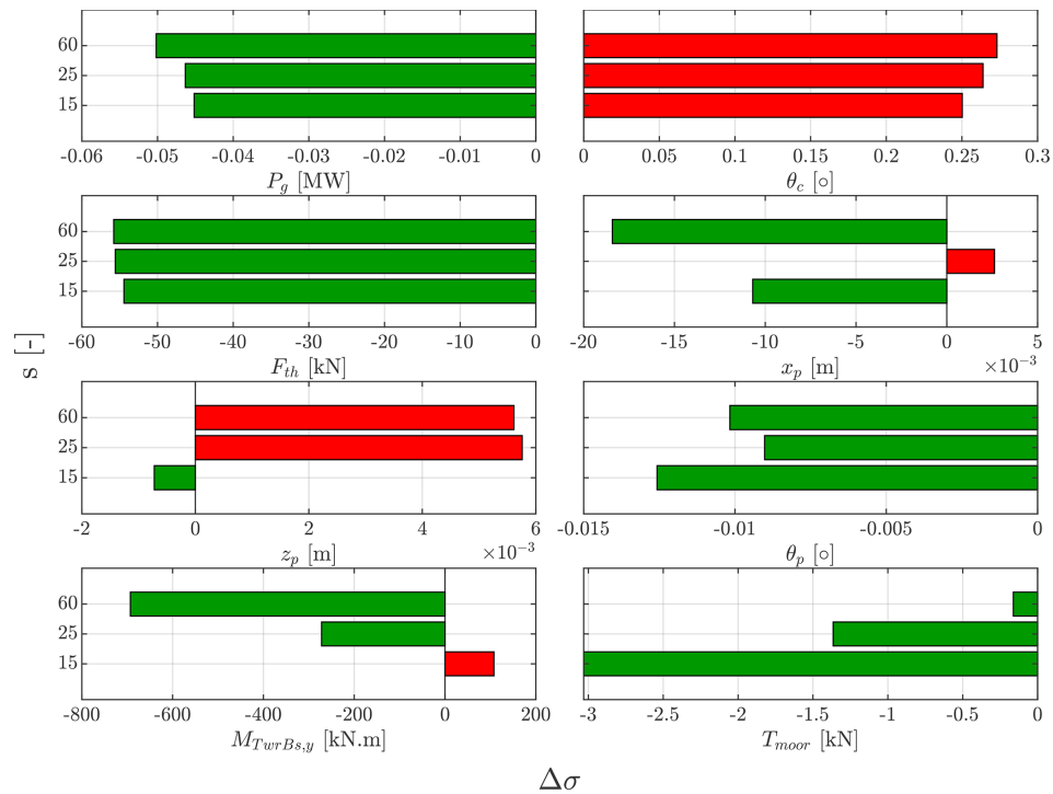
Figure 19. Normalized standard deviation percentage change of different variables of interest with wave FF control, at a turbulent wind speed of V = 14 \text{ m s}^{-1} with \text{TI} = 7.1 \% , and waves with H_s = 7 \text{ m} and T_p = 12 \text{ s} but with a different directional spreading parameter, S , varying from short-crested at s = 15 to longer-crested waves at s = 60 . The bars illustrate the difference in standard deviation with the FF control compared to the baseline case at each directional spreading parameter.
