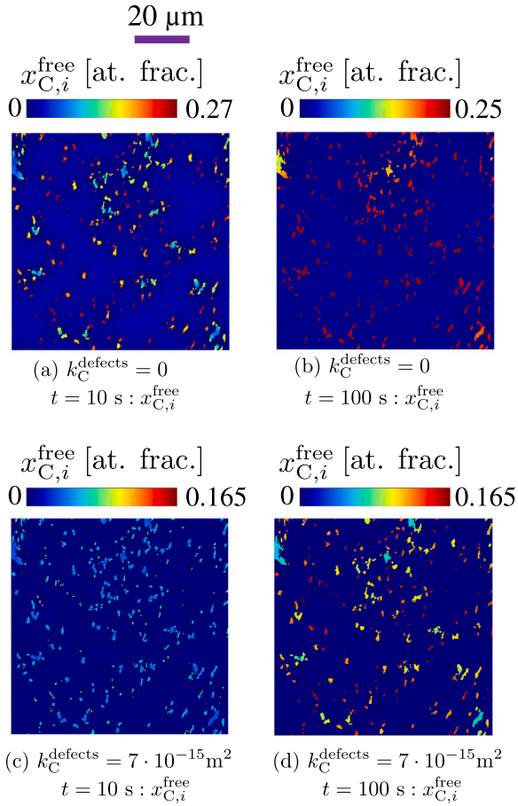
Fig. 11. Simulations of annealing at 400 °C with and without the consideration of trapping at defects, for a microstructure with f^\gamma = 0.05 .
