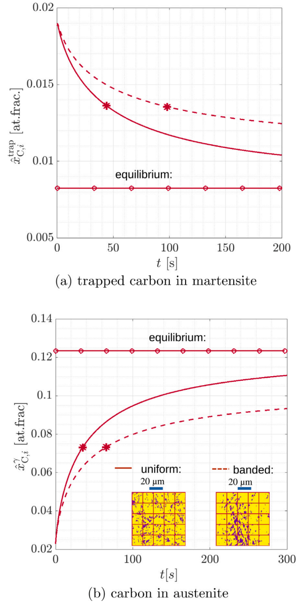
Fig. 14. Simulated outcome of average carbon concentration (a) segregated to martensite defects, and (b) in austenite, during annealing at 400 °C for different microstructures of the same austenite fraction; The asterisks indicate the half-times, namely (a) the de-trapping 44 s and 98 s, and (b) the austenite enrichment 35 s and 66 s, for the homogeneous and heterogeneous microstructure, respectively.
