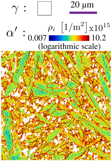
Fig. 8. Martensite-austenite microstructure ( f^\gamma = 0.10 ) obtained by EBSD. The map shows the phase (colored white if austenite) and defect density (if martensite).
