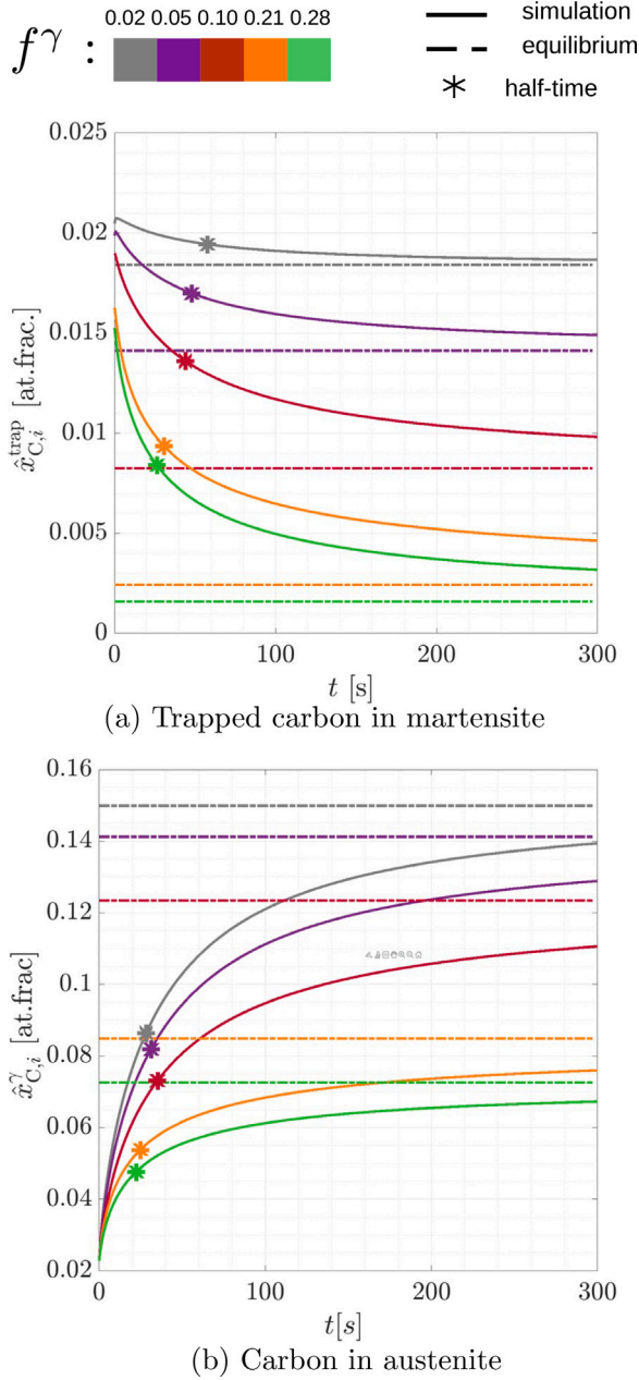
Fig. 13. Time evolution of carbon concentration redistribution; (a) shows the average carbon concentration in martensite defects and (b) the average carbon concentration in austenite, for simulations of annealing at 400 °C under the consideration of trapping to defects, for the microstructures of different austenite fraction. The asterisks indicate the half-life times t_{1/2} .
