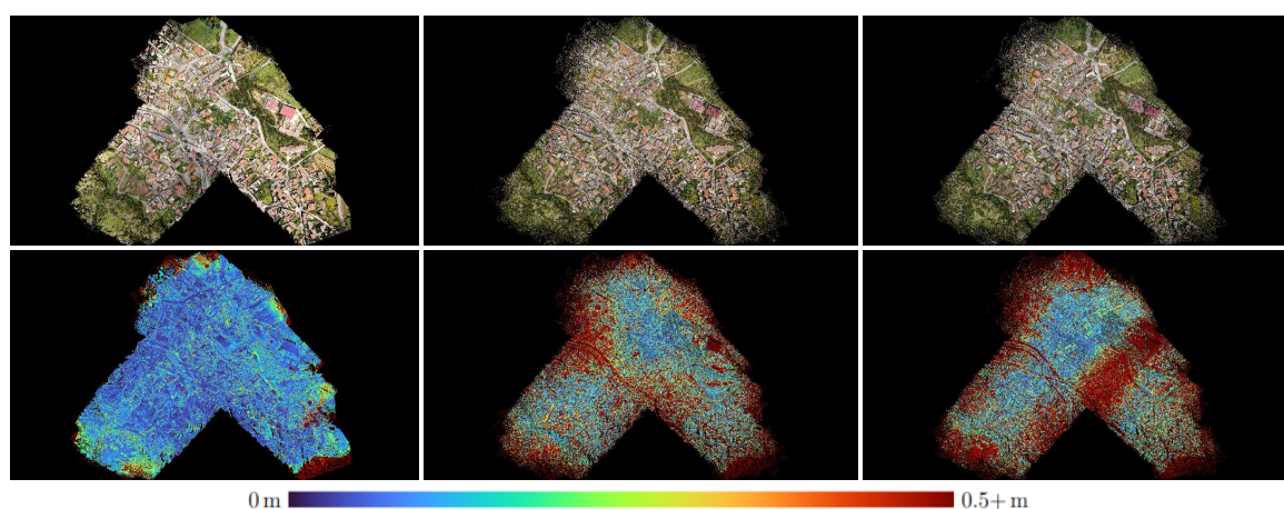
Figure 3. Colored point clouds (top) and their deviation from the LiDAR point cloud (bottom) for the 3D reconstructions achieved by COLMAP (left), Nerfacto-default (center) and Nerfacto-big (right) for Dataset-2.
