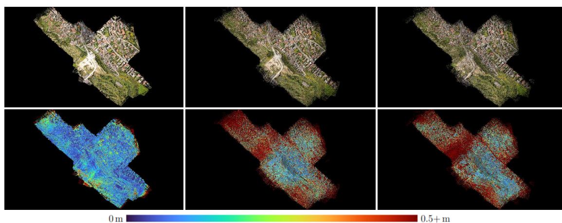
Figure 4. Colored point clouds (top) and their deviation from the LiDAR point cloud (bottom) for the 3D reconstructions achieved by COLMAP (left), Nerfacto-default (center) and Nerfacto-big (right) for Dataset-3.
