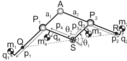
Fig. 1. Planar shaking force balanced pantograph consisting of four moving elements with a common center of mass located in base point S for any motion of the linkage [10].
