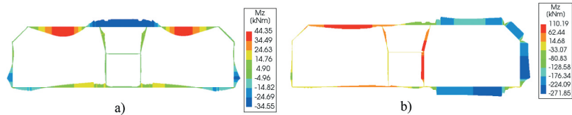
Figure 9. Bending moment diagrams for 2D plane strain representation: a) from mechanical loads b) at 365 minutes in fire scenario A.
