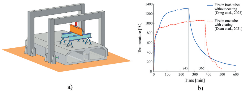
Figure 2. A) Setup during testing; b) fire scenarios for the tunnel segments tested by Dong et al. (2023) and Duan et al. (2021).
