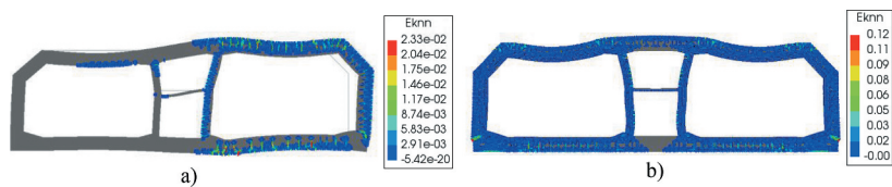
Figure 7. Comparison of crack patterns at the end of the heating phase for plane stress representation: a) scenario A; b) scenario B with explicit spalling representation. The numerical crack width can be estimated as w = \varepsilon \cdot h , with h = 30 mm.
