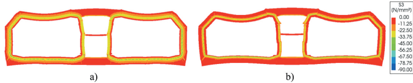
Figure 8. Principal compressive stresses for scenario B: a) plane strain and no spalling at 365 minutes; b) plane strain with explicit spalling at 72 minutes.
