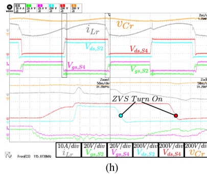
FIGURE 19. Experimental results for the different operating modes with 1.75 kW load power. (a) Designed converter prototype. (b) Experimental results for capacitive phase shift mode. (c) Power analyzer results for capacitive phase shift mode. (d) Experimental results for inductive phase shift mode. (e) Power analyzer results for inductive phase shift mode. (f) Experimental results for capacitive duty cycle mode. (g) Power analyzer results for capacitive duty cycle mode. (h) Experimental results for inductive duty cycle mode. (i) Power analyzer results for inductive duty cycle mode.
