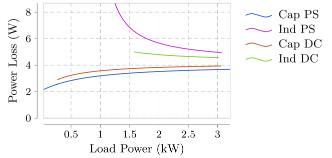
FIGURE 14. Switch turn-off losses for all the modes.
