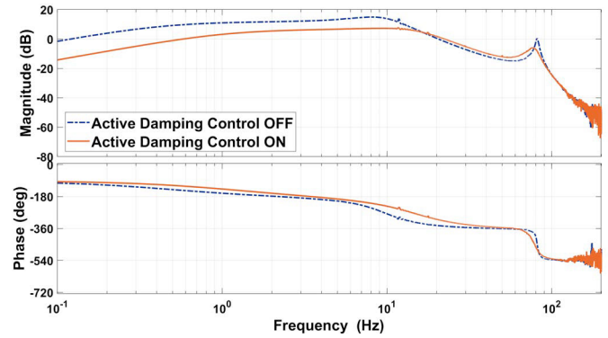
Fig. 6. Closed-Loop Experimental Process Sensitivity Frequency Response
