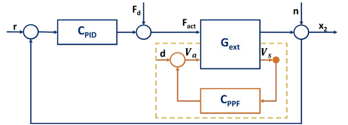
Fig. 2. Control Architecture implementing Active Damping Control
