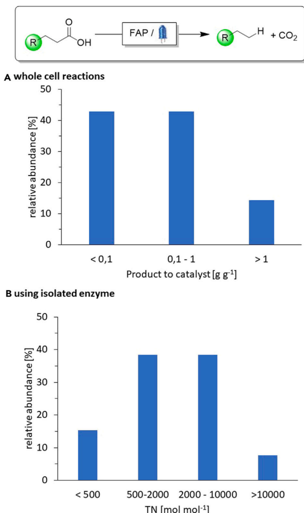
Figure 14. Catalyst performance of some representative FAP-catalyzed decarboxylation reactions
