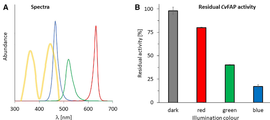
Figure 15. Photochemical properties of CvFAP
