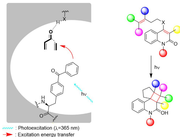
Figure 18. Creation of an artificial photoenzyme by incorporating a non-natural benzophenone amino acid and use of this for the stereoselective intramolecular Diels-Alder reaction
