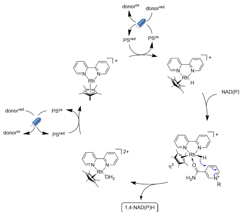
Figure 20. Using [\text{Cp}^*\text{Rh}(\text{bpy})(\text{H}_2\text{O})]^{2+} as catalyst for the selective reduction of \text{NAD(P)}^+ into enzyme-active 1,4-NAD(P)H
