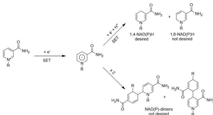
Figure 19. Direct reduction of \text{NAD(P)}^+ leads to significant amounts of undesired side products
