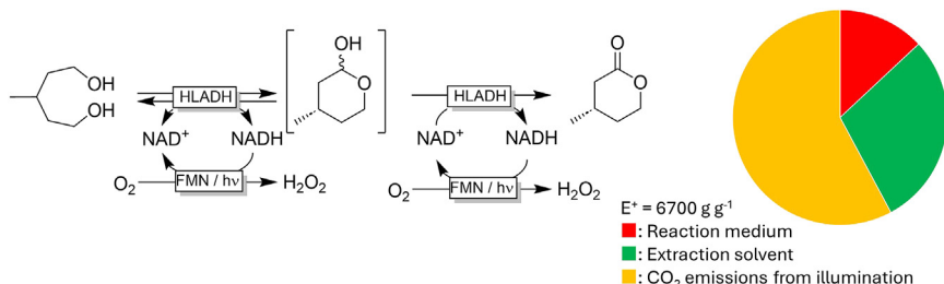
Figure 5. Estimation of the E^* factor of a photobiocatalytic oxidative lactonization reaction
