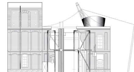
Elevation of one of the facades of the Textile museum, after adaptive reuse, with all the additions ( https://rb.gy/fzatpe )
