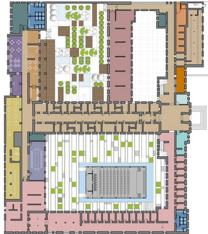
One of the floor plans of Qasr Garden Museum, after adaptive reuse (EBA[M] Architects, https://rb.gy/lhvw9j )
