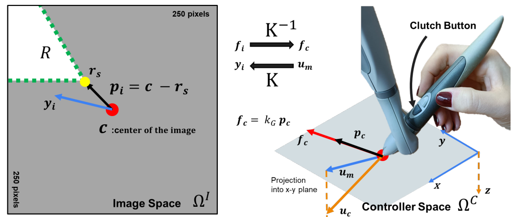
Figure 3. GVF coordinate transformation between the image space \Omega^I (Left) and controller space \Omega^C (Right) by the scaling transformation matrix K . Both the teleoperating manipulation and the GVF rely on the information in \Omega^I . To link \Omega^I with \Omega^C , u_c in \Omega^C are projected into x - y plane to form u_m . Using space transformation matrix K , u_m is transformed into desired target movement, y_i , in \Omega^I . Reversely, the guidance vector, p_i created by GVF in \Omega^I can be also transformed into \Omega^C as p_c using K^{-1} . In the top figure, R is the set of two-dimensional vectors of the segmented route. c , r_s , and p_i is the center of the image, the closest point in R to c , and the guidance vector, respectively.
