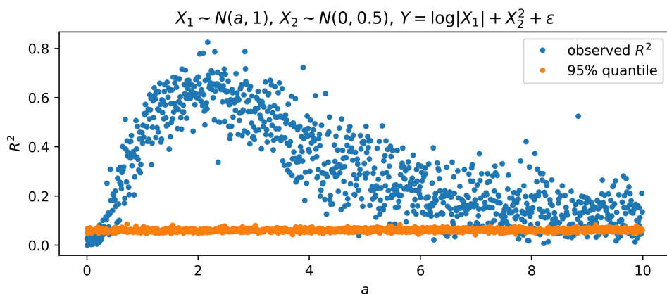
(a) The plot shows the results of performing the permutation test for linear regression model with the class of functions \mathcal{F}_{\text{LR}} . The sample size is 100. The blue dots show the observed R^2 and the orange dots show the 95% quantile of the empirical distribution of generated R^2 (approximation using 200 permutations). The test has been performed for values of a ranging between 0 and 10.
