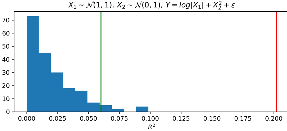
(a) Histogram of the distribution of generated R^2 using permutation of y values. The model considered here is linear regression with the class of functions \mathcal{F}_{\text{LR}} . The sample size is 100. The red line denotes the observed R^2 for the true pairings of X and Y , the green line denotes the 95%-quantile of the empirical distribution of R^2 (approximation using 200 permutations).
