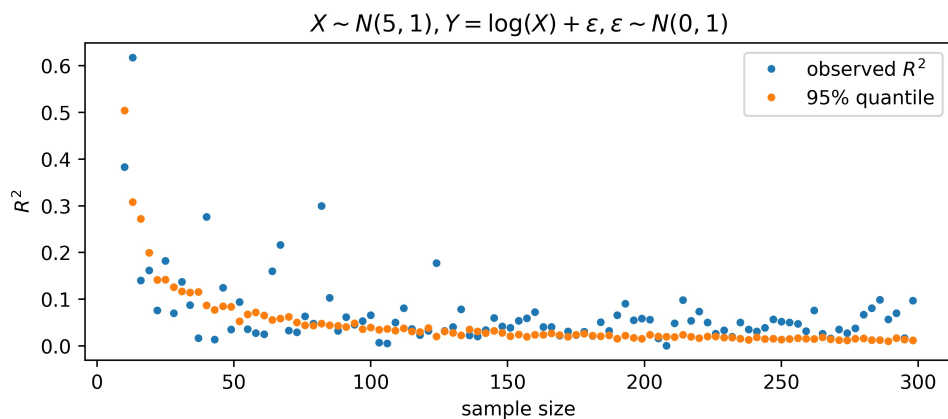
(a) The plot shows the results of performing the permutation test for linear regression model with the class of functions \mathcal{F}_{\text{LR}} . The blue dots show the observed R^2 and the orange dots show the 95% quantile of the empirical distribution of generated R^2 (approximation using 200 permutations). The test has been performed for sample sizes ranging between 10 and 300.
