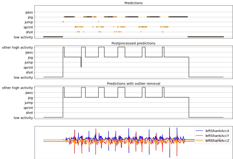
Figure 2.20: Example 2 of final results. True labels: jog and turn 5 times with a final jog.
