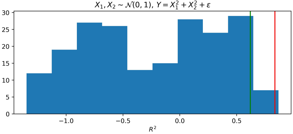
Figure 5.1: Histogram of the distribution of generated R^2 using permutation of y values. The model considered here is a 3-layered neural net. The sample size is 10. The red line denotes the observed R^2 for the true pairings of X and Y , the green line denotes the 95%-quantile of the empirical distribution of R^2 (approximation using 200 permutations).
