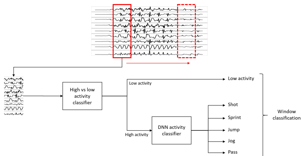
Figure 2.13: Sliding window evaluation diagram.
