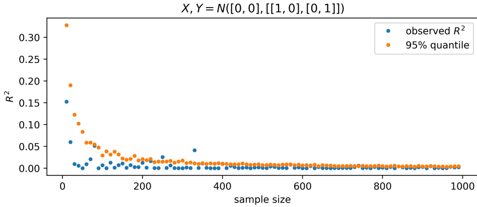
(a) The plot shows the results of performing the permutation test for linear regression model with the class of functions \mathcal{F}_{\text{LR}} . The blue dots show the observed R^2 and the orange dots show the 95% quantile of the empirical distribution of generated R^2 (approximation using 200 permutations). The test has been performed for sample sizes ranging between 10 and 1000.
