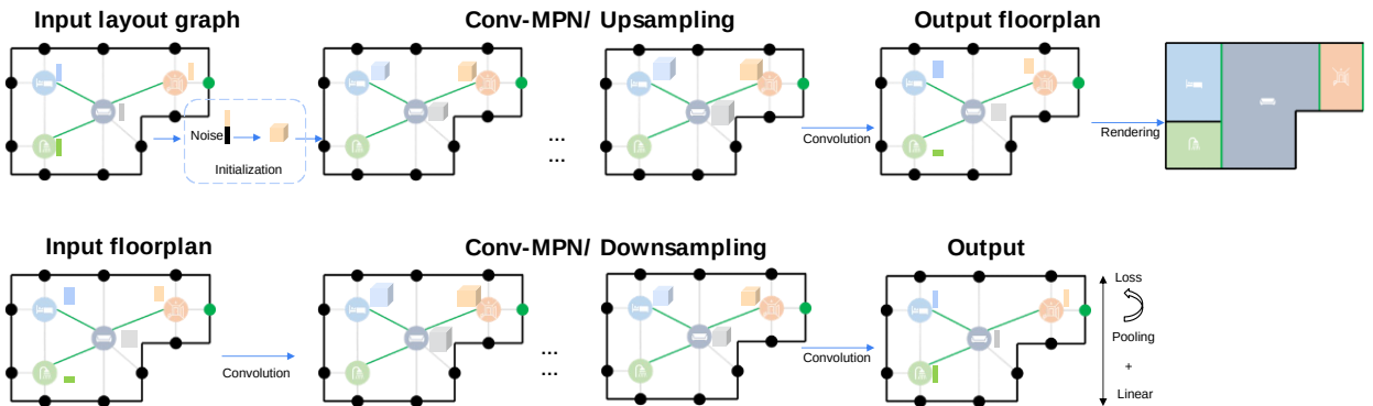
Figure 4 Floorplan generator (top) and discriminator (bottom). ConvMPNI is our backbone architecture [9]. The input graph constraint is encoded into the graph structure of their relational networks.
