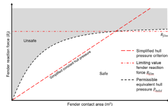
Figure 7 Maximum fender reaction force (Berendsen et al., 2024) [2].
