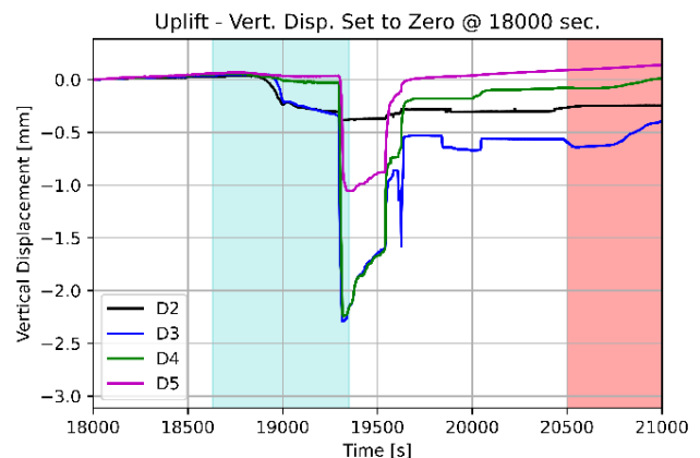
Figure 6. Vertical displacements measured by the DCDTs at the initiation of uplift.
