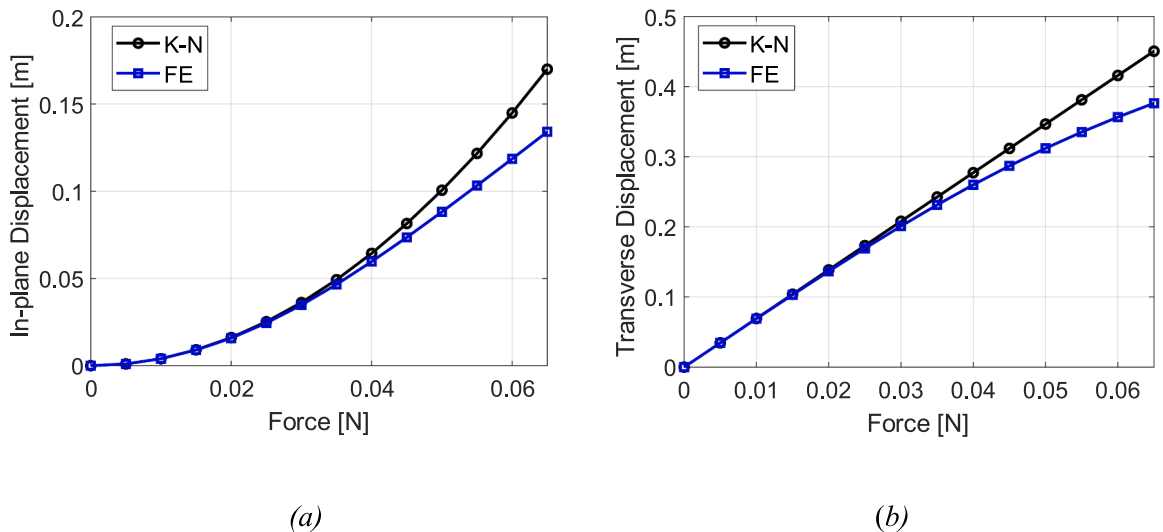
Fig 1. Peak displacements in steady state solutions of a steel cantilever beam of length l = 0.6931 m, b = 0.0254 m, d = 0.99 mm compared at different load amplitudes – (a) in-plane displacements, (b) transverse displacements.
