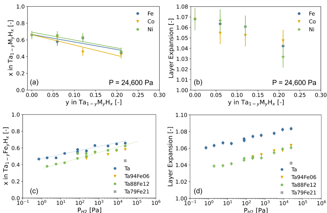
Figure 4. In situ NR results of the 40 nm \text{Ta}_{1-y}\text{Fe}_y , \text{Ta}_{1-y}\text{Co}_y , and \text{Ta}_{1-y}\text{Ni}_y thin films with a 4 nm Ti adhesion layer and capped with 10 nm \text{Pd}_{0.6}\text{Au}_{0.35}\text{Cu}_{0.05} at T = 22^\circ\text{C} . A selection of the data with the corresponding fits and SLD profiles can be found in Figures 3 and S15. (a) Fe/Co/Ni concentration dependence of the amount of hydrogen absorbed by the \text{Ta}_{1-y}\text{M}_y\text{H}_x layer at P_{\text{H}_2} = 24,600 Pa. (b) Fe/Co/Ni concentration dependence of the relative layer expansion of the \text{Ta}_{1-y}\text{M}_y\text{H}_x layer at P_{\text{H}_2} = 24,600 Pa. (c) Hydrogen pressure dependence of the amount of hydrogen absorbed by the \text{Ta}_{1-y}\text{Fe}_y\text{H}_x layer. (d) Hydrogen pressure dependence of the expansion of the \text{Ta}_{1-y}\text{Fe}_y layer. The lines are an ordinary least-squares fit to the data.
