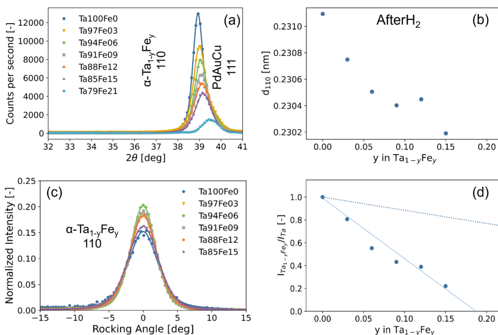
Figure 2. Ex situ X-ray diffraction (XRD) results of the 40 nm Ta 1-y Fe y thin films with a 4 nm Ti adhesion layer and a 10 nm Pd 0.6 Au 0.35 Cu 0.05 capping layer after exposure to hydrogen and measured in air. (a) Diffraction patterns (Cu Kα, λ = 0.1542 nm) of the Ta 1-y Fe y thin films. The continuous lines represent fits of two pseudo-Voigt functions to the experimental data to account for the bcc(110) Ta 1-y Fe y and fcc(111) Pd 0.6 Au 0.35 Cu 0.05 peaks. (b) Fe concentration dependence of the d 110 spacing in Ta 1-y Fe y . The continuous line is an ordinary least-squares fit to the data. (c) Rocking curves of the Ta 1-y Fe y thin films around the bcc Ta 1-y Fe y (110) peak. In this figure, the intensity is normalized to the integrated intensity across all rocking angles. (d) Fe concentration dependence of the total intensity of the (110) diffraction peak in Ta 1-y Fe y , by taking into account the effect of both the changing amplitude and width. The intensity is computed by multiplying the integrated intensity of the fitted (110) Ta 1-y Fe y peak by the fwhm of the rocking curve of (b). The intensity is subsequently scaled to the intensity of the Ta sample. The continuous line indicates an ordinary least-square fit to the data and the dashed line indicates the theoretically expected Fe concentration dependence of the intensity according to eq 2.
