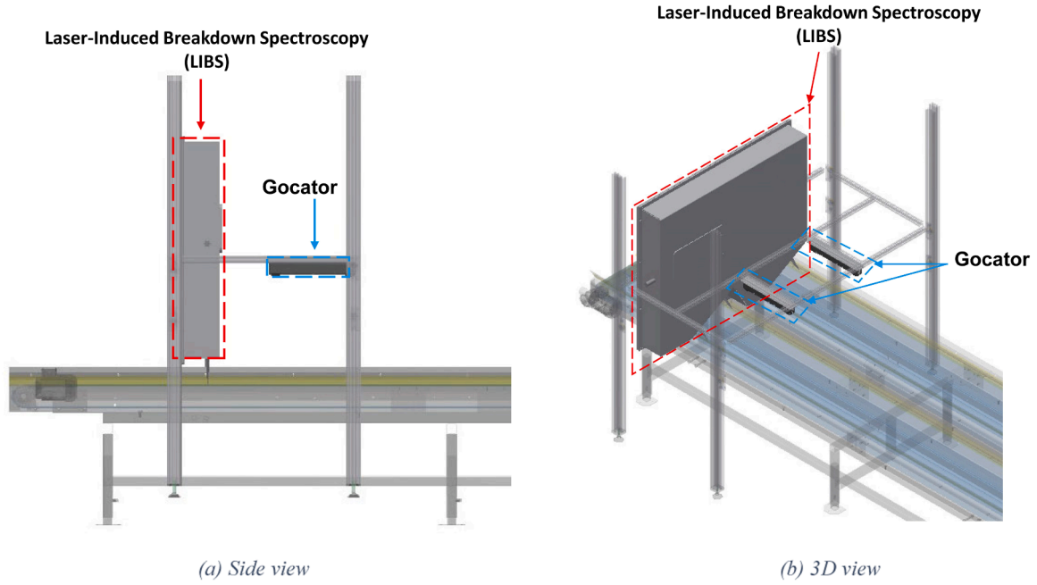
Fig. 4. Pre-calibrated sensors.
