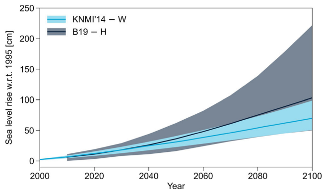
Figure 7. Projections of SLR along the Dutch coast for the W scenario of KNMI'14 and the H scenario of Bamber et al. (2019). Lines represent the median values, and the bandwidth depicts the 5th–95th percentile range of the projections.
