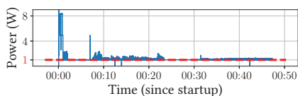
Figure 2: Sunlight collector's power consumption.
