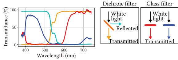
Figure 6: Spectral response of dichroic filters used at the transmitter (turquoise and orange) and glass filters used at the receiver (blue and red).
