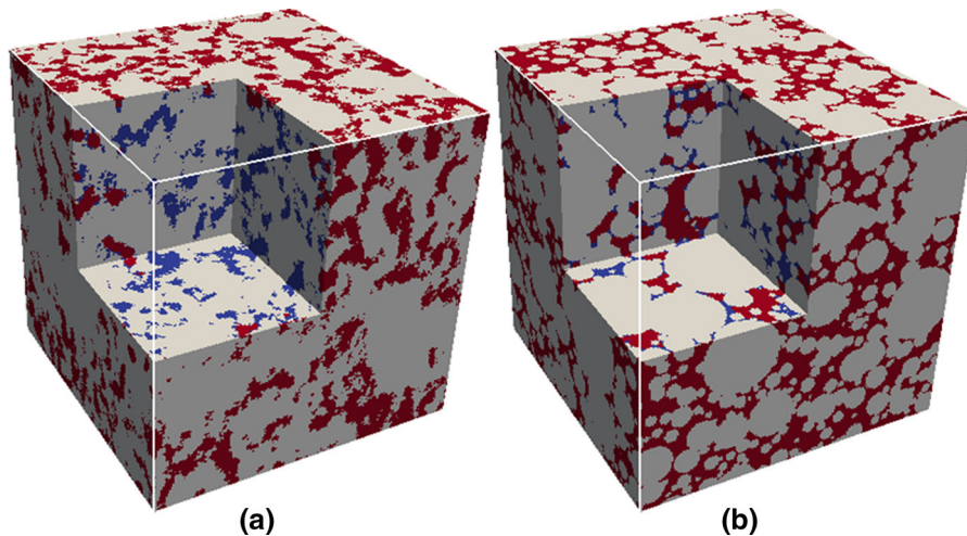
Fig. 7 Visualization of differentiated pores in CT-1d (MIP simulation). Corresponding pore size d_c is 2 \mu\text{m} , with mercury-intruded pores in red, empty pores in blue and the solid phase in white
