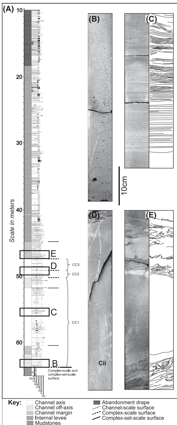
Figure 5. (A) Core log through subunit C2 in borehole Bav 2. (B) Fine-grained sandstone with mudstone clasts dispersed throughout the entire 1-m (3-ft) section (location of core photograph shown on core log A). (C) Core photograph and interpretation showing an upward progression from structureless fine-grained sandstone to planar lamination followed by climbing ripple lamination. (D) Structureless fine sandstone with a mudclast mantled channel base at the top of the core interval. (E) Deformed and dewatered fine-grained sandstone showing a well-developed loaded basal contact and an upper deformed sandstone and siltstone zone. CC1 = channel complex 1; CC2 = channel complex 2; CC3 = channel complex 3; Csi = coarse-grained siltstone; fs = fine-grained sandstone; Fsi = fine-grained siltstone; ms = medium-grained sandstone; Msi = medium-grained siltstone; Mud = mud grade sediment; vfs = very fine-grained siltstone.
