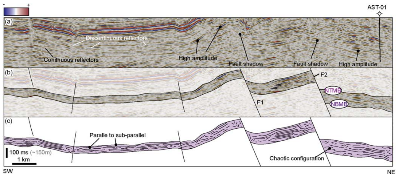
Figure 8. Un-interpreted (a) and interpreted (b–c) 2D seismic profile 80-03 (see location on Fig. 2) showing the main geometries in the Main Buntsandstein observed around AST-01. See text for detail description of the seismic profile.
