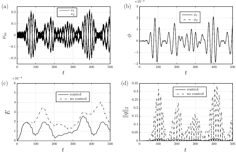
Figure 21: Closed-loop performance for the multiple frequency disturbance case. Controller (II) with low sensor noise is considered. (a) Shear measurements \nu_m used for feedback. (b) Control input \phi . (c) Perturbation energy E = \|\mathbf{u}\|_{L^2}^2 . (d) Norm of the controlled perturbation shear output \|\mathbf{q}\|_2 .
