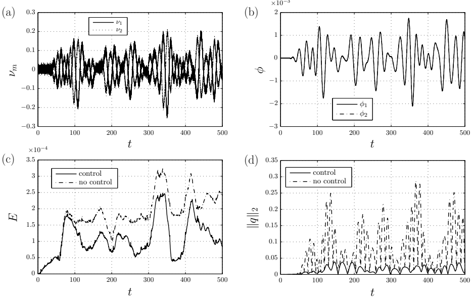
Figure 25: Closed-loop performance for the stochastic disturbance case. Controller (II) with low sensor noise is considered. (a) Shear measurements \nu_m used for feedback. (b) Control input \phi . (c) Perturbation energy E = \|\mathbf{u}\|_{L^2}^2 . (d) Norm of the controlled perturbation shear output \|\mathbf{q}\|_2 .
