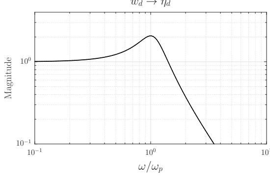
Figure 2: Magnitude plot of the low pass filter (2.12) used for the disturbance model. The frequency is normalized with the peak frequency \omega_p .
