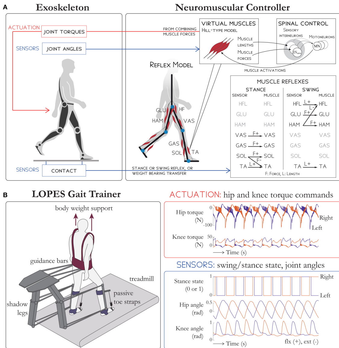
FIGURE 1 | Schematic overview of (A) the NMC and (B) the LOPES gait trainer. (A) Sensors on the exoskeleton are used to detect ground contact. Then, depending on whether the limb is in stance or swing, different reflex rules are activated (shown on the bottom right table). An extra term is added to the hip flexors HFL and hip extensors GLU to facilitate the weight bearing transfer during double support. The reflex loops (which use muscle length, stretching velocity, and tendon force) are then combined to stimulate virtual Hill-type muscles which then generate active torques on exoskeleton joints. (B) Subjects in LOPES walk on a treadmill with body weight support. Knee and hip actuation is provided with guidance bars moved by shadow legs, and passive toe straps prevents toe drag. The NMC provides hip and knee torque commands. Sensory input into NMC include stance state, hip angle, and knee angle for both legs. LOPES figure based on Meuleman et al. (2016).
