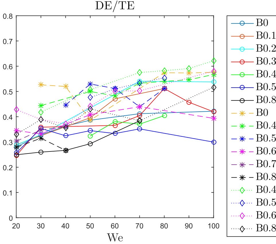
FIG. 8. The normalized viscous dissipated energy as a function of We for different B s and Ca s: Ca = 0.1 for continuous lines and circles, Ca = 0.5 for dashed lines and asterisks, Ca = 1 for dotted lines and diamonds.
