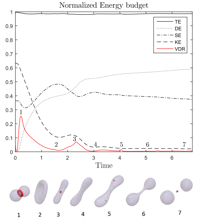
FIG. 6. Normalized energy budget of the kinetic energy KE, surface energy SE, dissipated energy DE, total energy TE for stretching separation at We = 90 , B = 0.4 , and Ca = 1 . The viscous dissipation rate VDR is given by the red line (note that an arbitrary vertical scaling was used). The time is normalized by d/v_{rel} .
