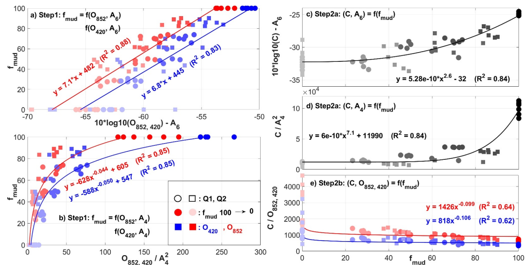
Figure 4. Application of SCI method to four optical/acoustic pairs with all data in Q set (Q12). The reductions of f_{\text{mud}} from 100% to 0% are shown by the darkest color to lightest color. Blue: data from O 420 . Red: data from O 852 . The displayed functions are obtained from data set Q12.
