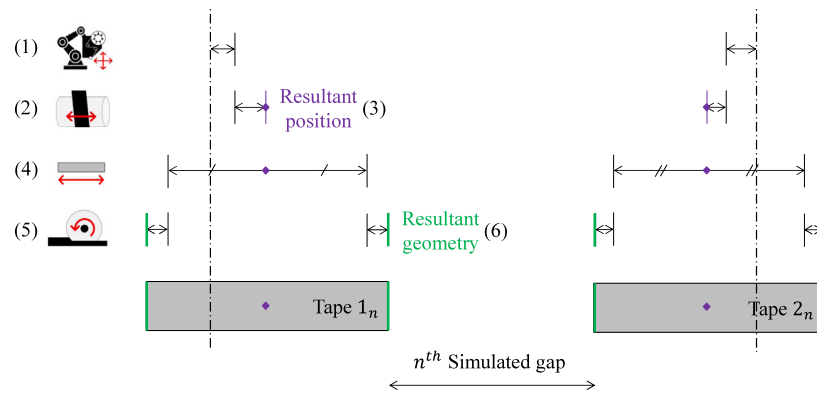
Fig. A.14. Schematic depicting the steps to simulate a tow section per the algorithm enumerated in this section. The dot-dashed lines represent the programmed tow-to-tow distance. Each double arrow line depicts a value drawn from a distribution fit. Two simulated adjacent tows and the resulting simulated gap is shown.
