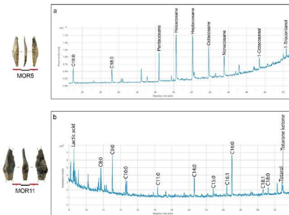
Figure 4.6: Partial chromatograms of MOR5 and MOR11 showing significant lipids preservation.
